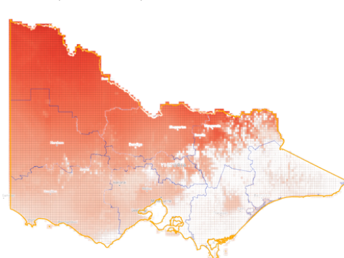
2090s (2075-2104)
